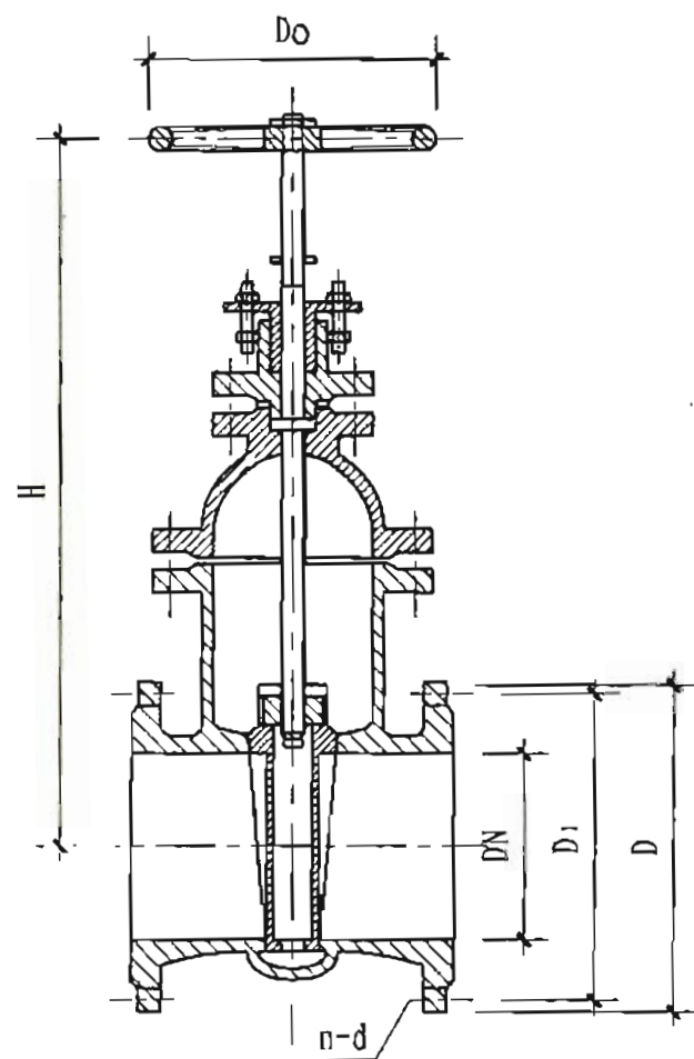
Z45 T W -10型暗杆楔式闸阀
