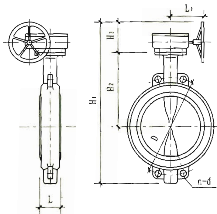
PD371F-25Q型蜗轮传动偏心式蝶阀
