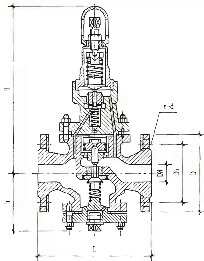
Y43H-16型活塞式减压阀
