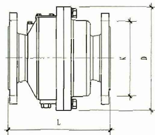
W-TZCY41-16Q型 (DN40-DN150)
