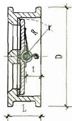
蝶形双门消声止回阀
